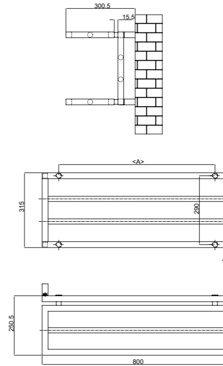
SMART U nipped/niplat ( for chrome plated/ pentru cromat)
